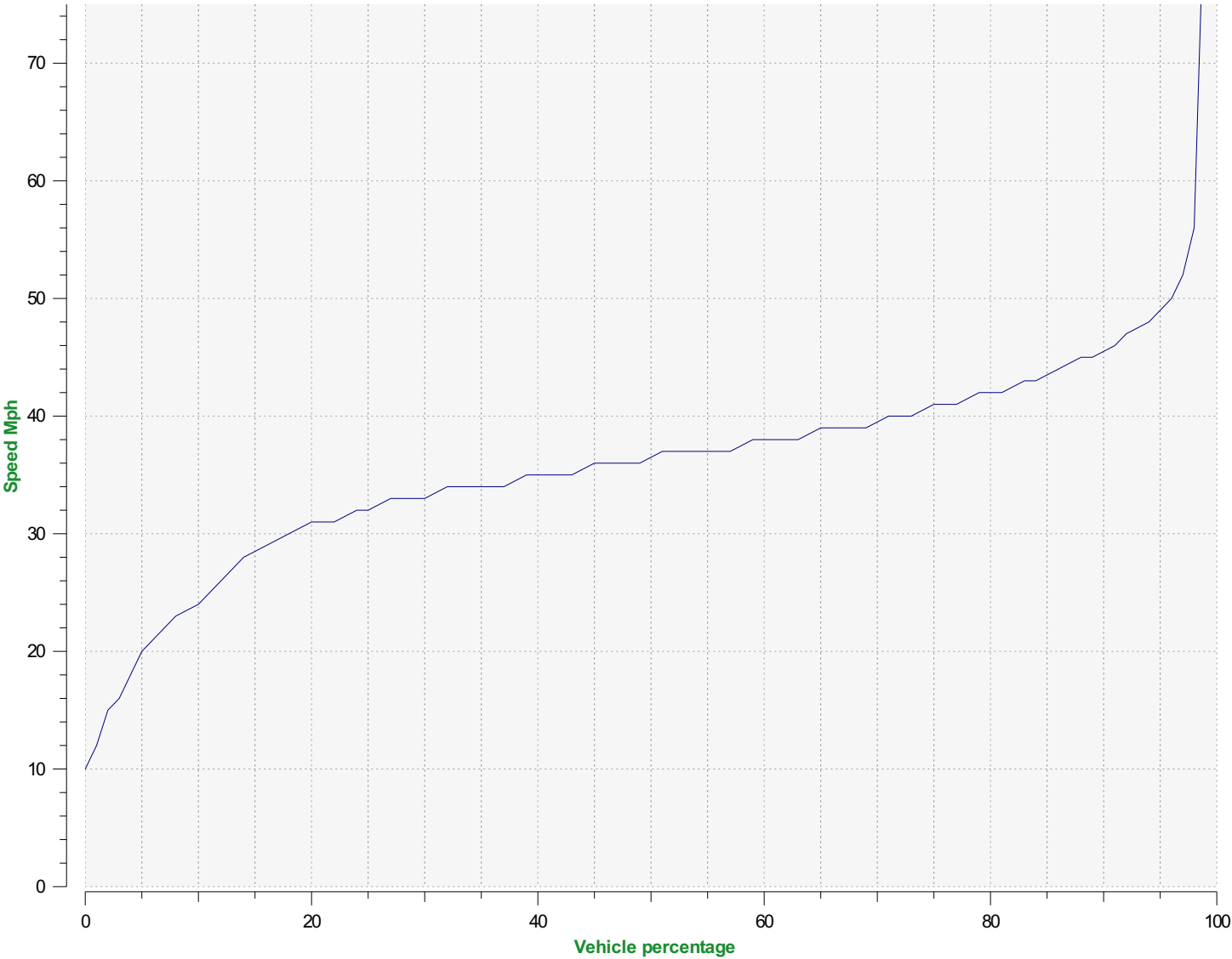
Speed percentile(outgoing)
